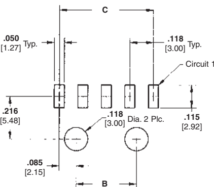
Recommended PC Board Layout* 4-12 Positions
