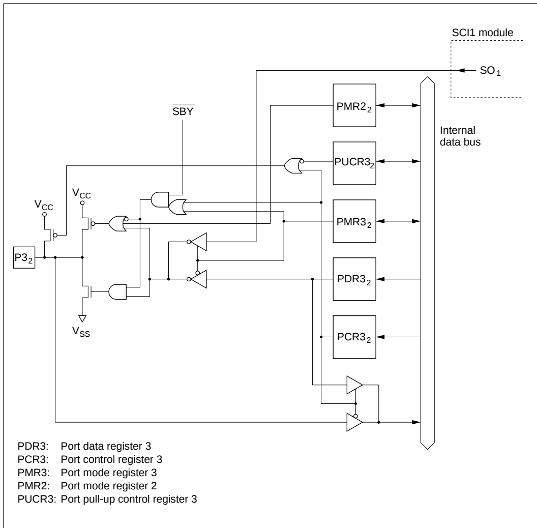
Figure C-3 (b) Port 3 Block Diagram (Pin P3 2 )
