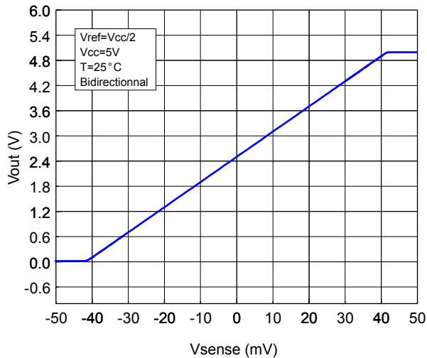
Figure 19. (Output voltage + V_{ref} ) vs. V_{sense} bidirectionnal with V_{CC} = 5\text{ V}
