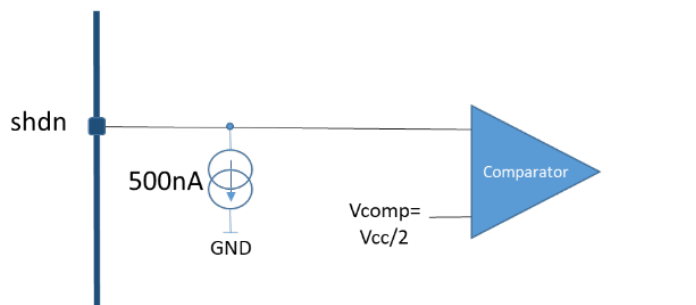
Figure 64. SHDN pin
