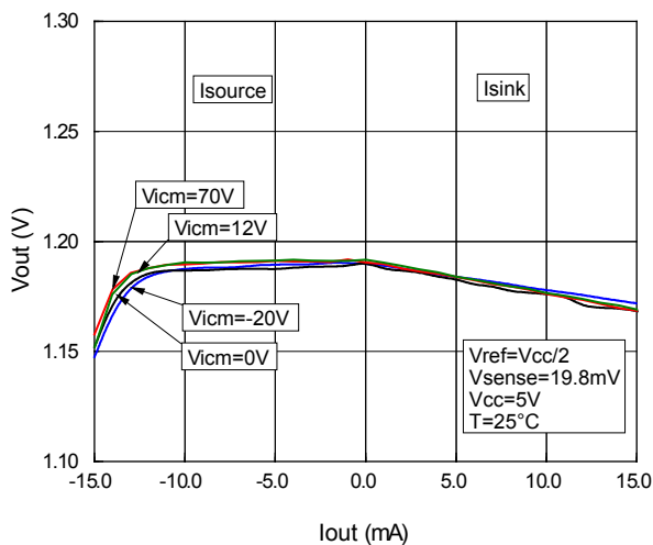
Figure 25. Load regulation with V_{CC} = 5\text{ V}
