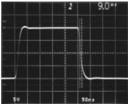
R_F = R_G = 750\Omega V_S = \pm 15\text{V} R_L = 10\Omega 1210 F05b
