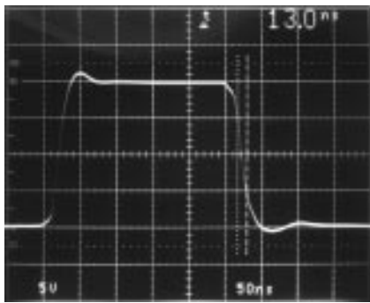
R_F = 825\Omega V_S = \pm 15\text{V} R_L = 10\Omega 1210 F05a
