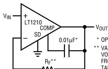
Buffer A_V = 1
