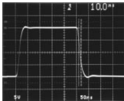
R_F = R_G = 750\Omega V_S = \pm 15\text{V} R_L = 10\Omega 1210 F05c
