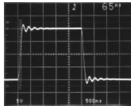
R_F = R_G = 3\text{k} V_S = \pm 15\text{V} R_L = \infty 1210 F06
