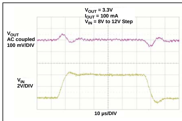
FIGURE 2-20: Line Transient Response.
