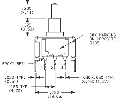
8161SH9_BE2 SPDT
