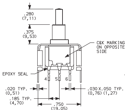
8261SH9_BE2 DPDT
