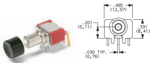
8161SH9ABE2 SPDT
