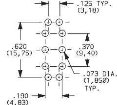
8261SH9_BE2 DPDT
