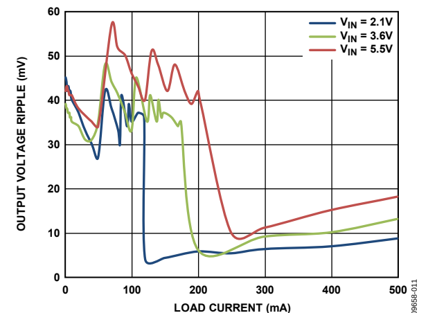
Figure 10. Output Voltage Ripple vs. Load Current
