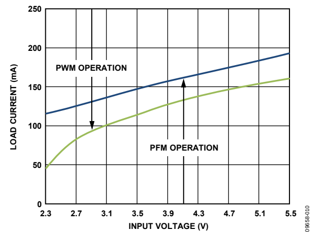
Figure 9. Auto Mode Switching Threshold vs. Input Voltage
