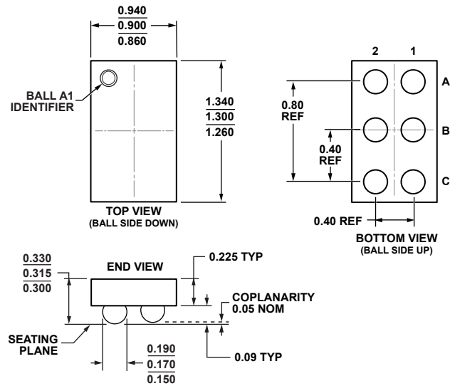
Figure 33. 6-Ball Bumped Bare Die Sales [BUMPED_CHIP] (CD-6-4)
