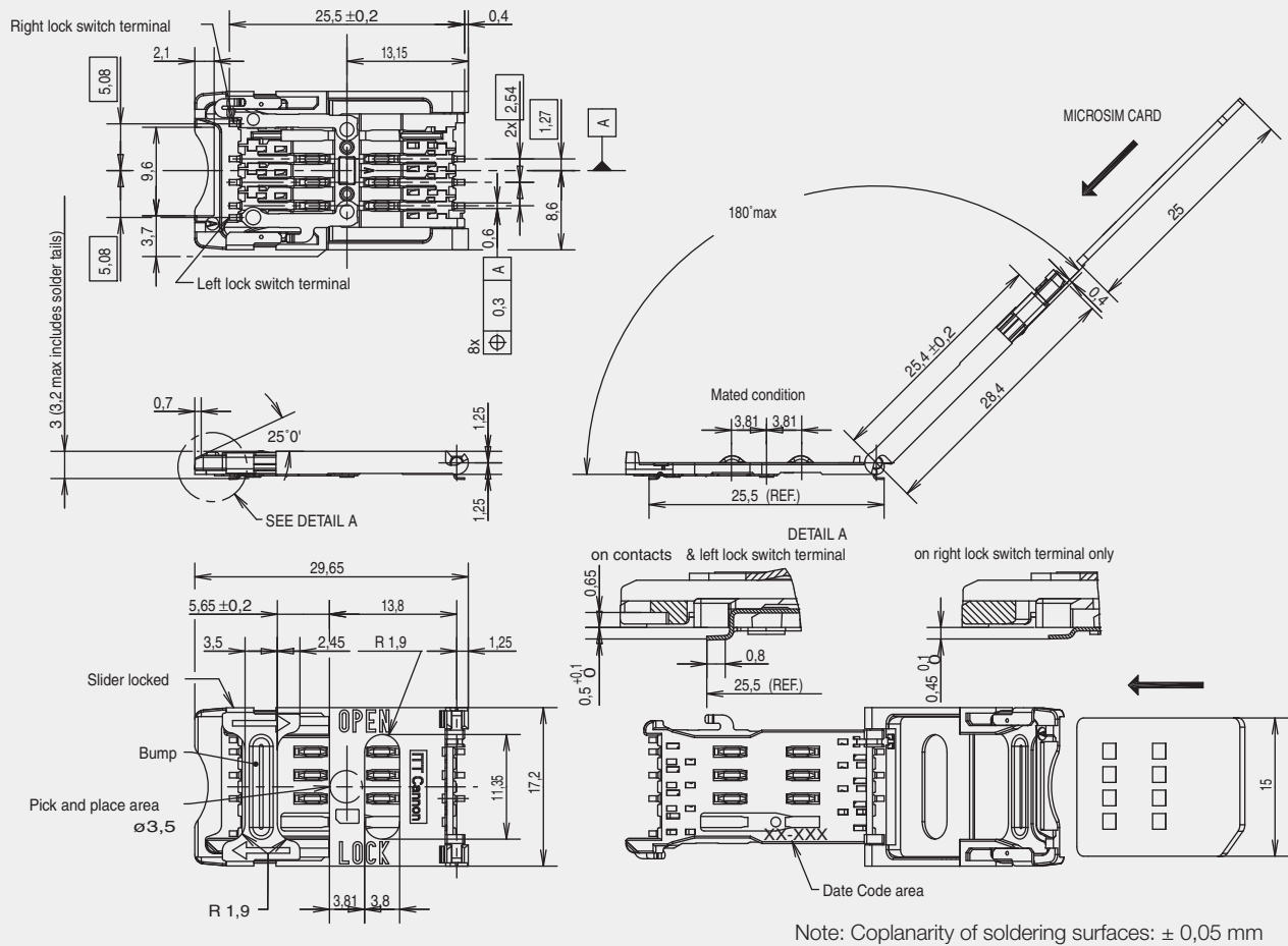
Hinged Cover CCM03 - 3514 (6 contacts - with switch on metal lock)
