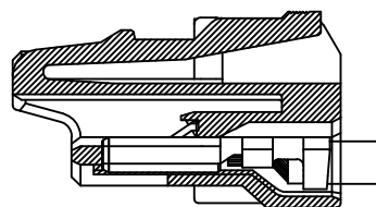
MATED WITH HEADER ASSEMBLY [REFERENCE]
