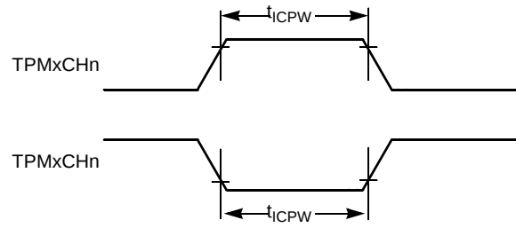
Figure 32. Timer Input Capture Pulse
