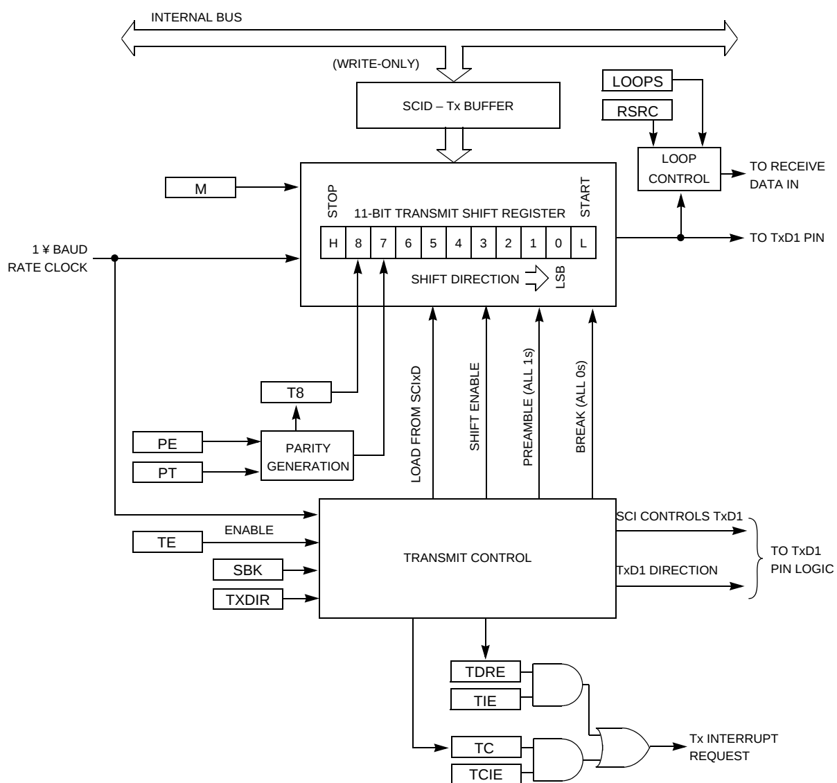
Figure 22. SCI Transmitter
