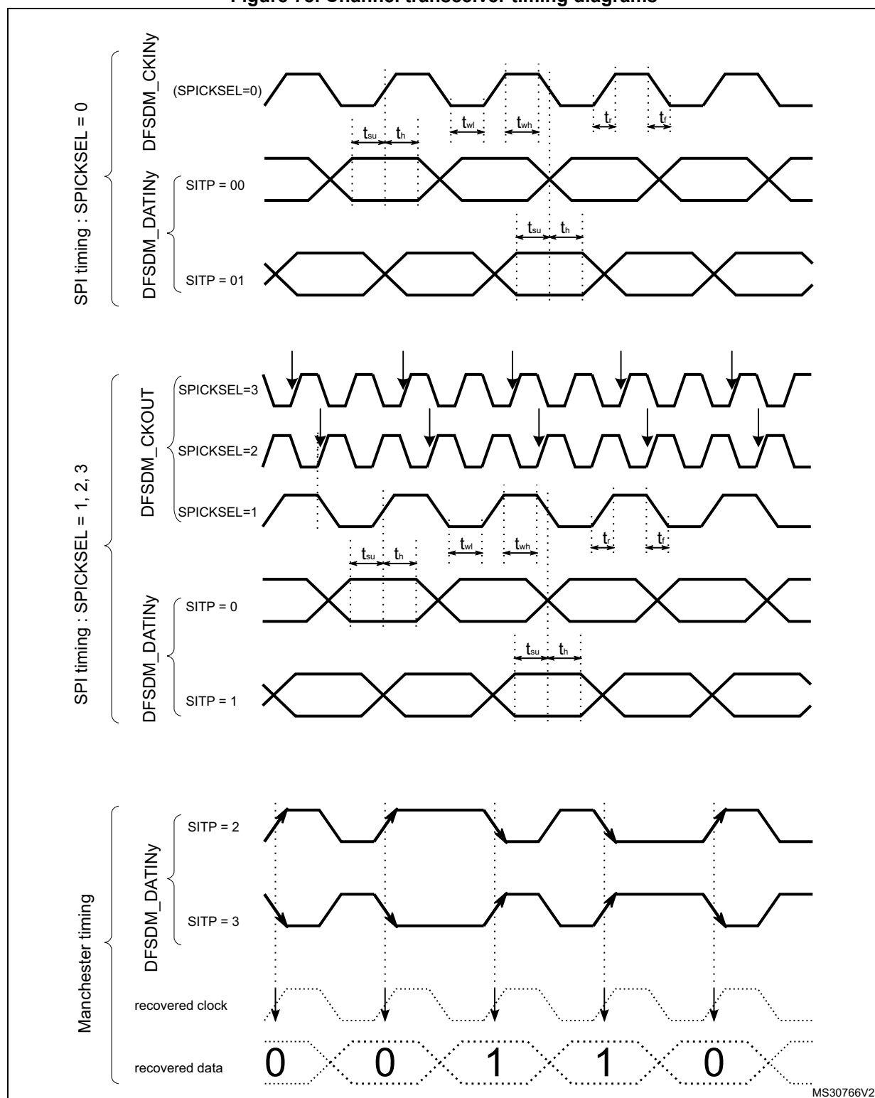
Figure 78. Channel transceiver timing diagrams
