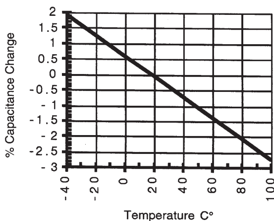
Capacitance Change vs. Temperature
