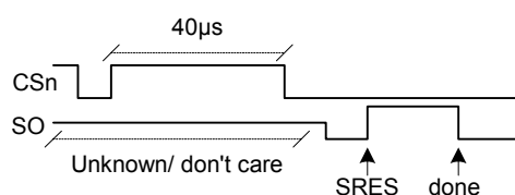
Figure 12: Power-on reset with SRES
