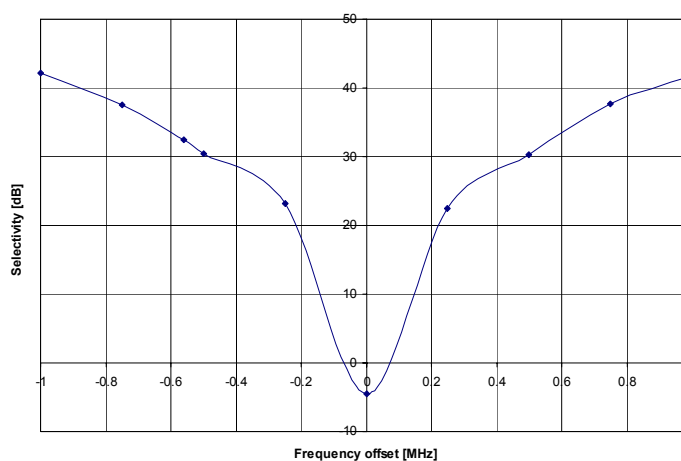
Figure 17: Typical selectivity at 2.4 kbps. IF frequency is 273.9 kHz.
