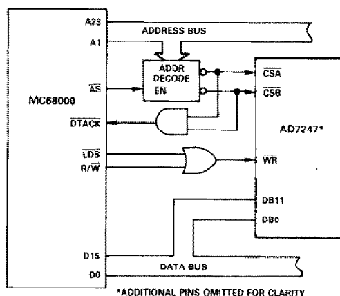
Figure 12. AD7247 to MC68000 Interface
