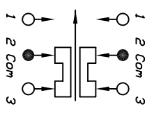
CIRCUIT: DPDT
