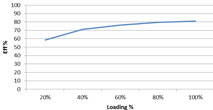
AM1D-1512SZ Efficiency vs. Loading
