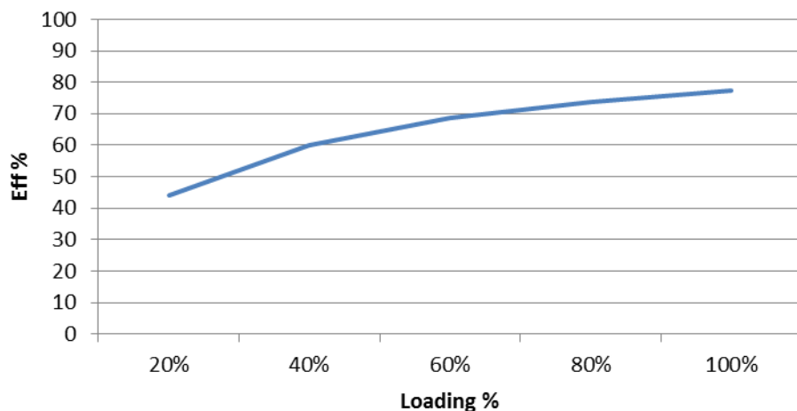
AM1D-4824SZ Efficiency vs. Loading
