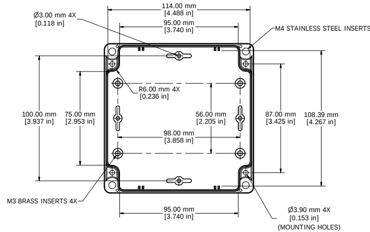
BOX - INSIDE
