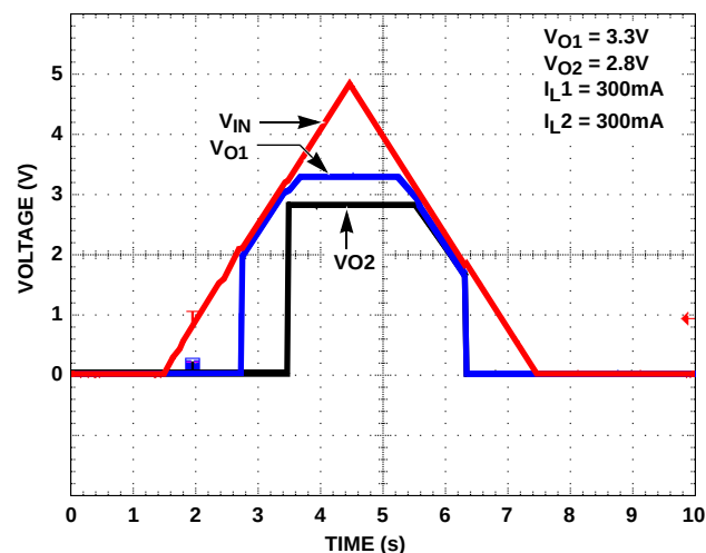
FIGURE 12. POWER-UP/POWER-DOWN
