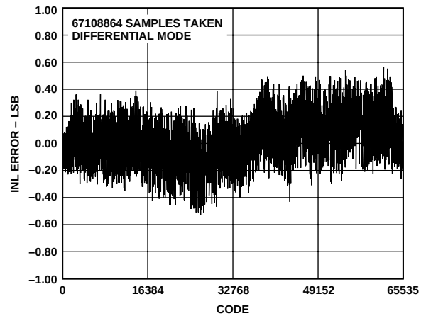
Figure 19. Integral Nonlinearity (Output Data Rate = 1.2 MHz)
