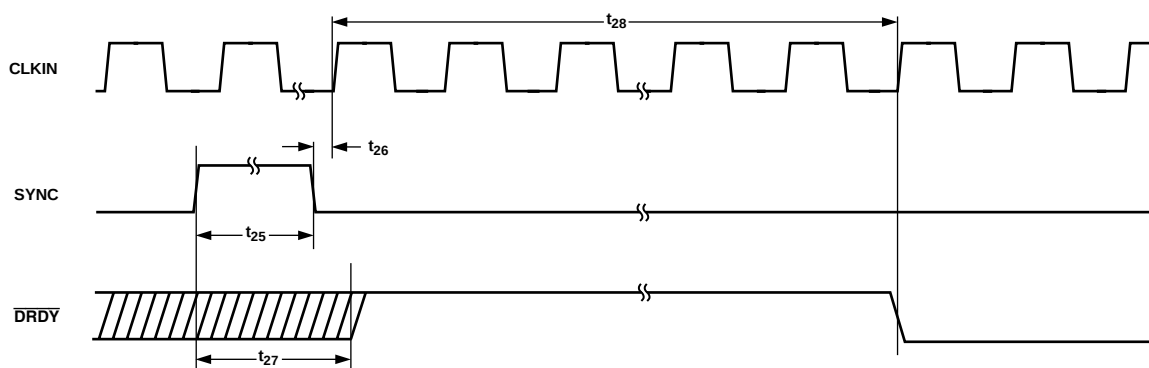
Figure 8. SYNC Timing
