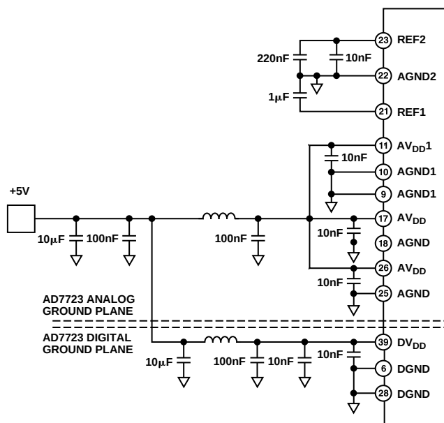
Figure 44. Reference and Power Supply Decoupling
