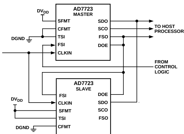
Figure 39. Serial Mode 1 Connection for Two-Channel Multiplexed Operation
