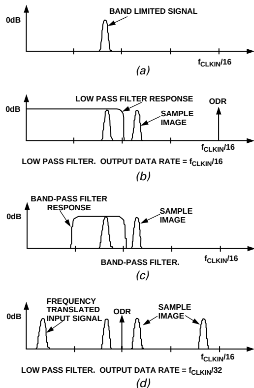
Figure 25. Band-Pass Operation
