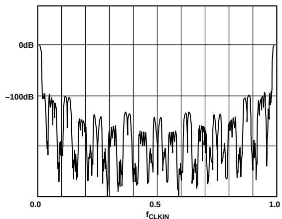
Figure 26b. Low-Pass Filter Decimate by 32
