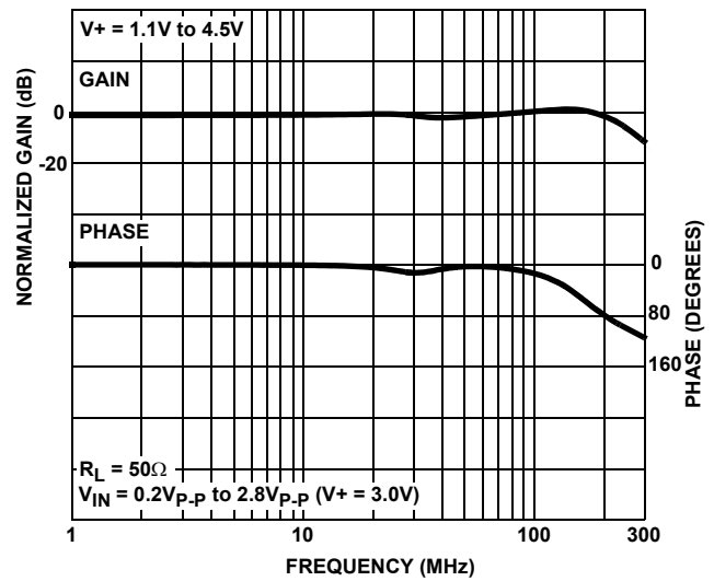
FIGURE 16. FREQUENCY RESPONSE
