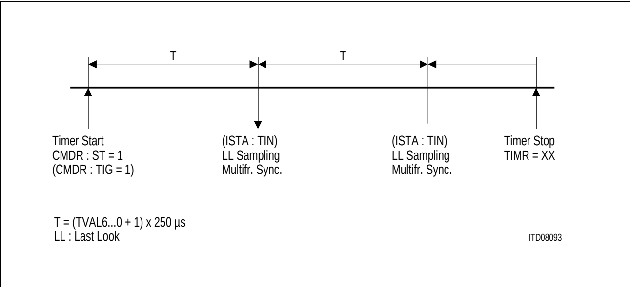
Figure 77 Timer Applications
