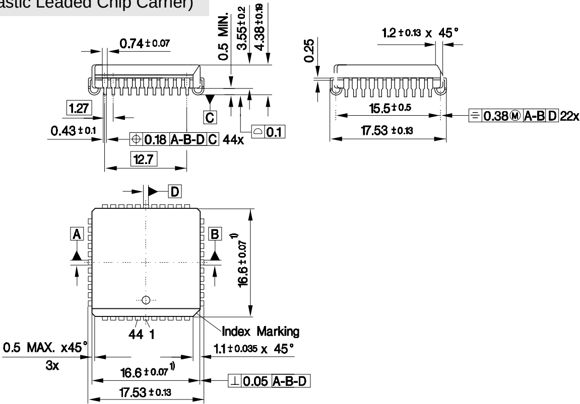
P-LCC-44-1 (Plastic Leaded Chip Carrier)
