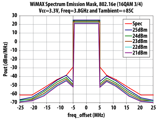
Figure 43. SEM at Vcc=3.3V, +85C and 3.8GHz over Vcc (2dB Post-PA loss assumed)
