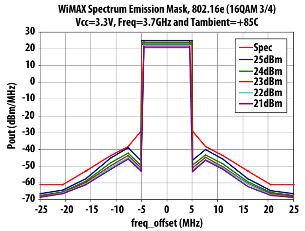
Figure 42. SEM at Vcc=3.3V, +85C and 3.7GHz over Vcc (2dB Post-PA loss assumed)
