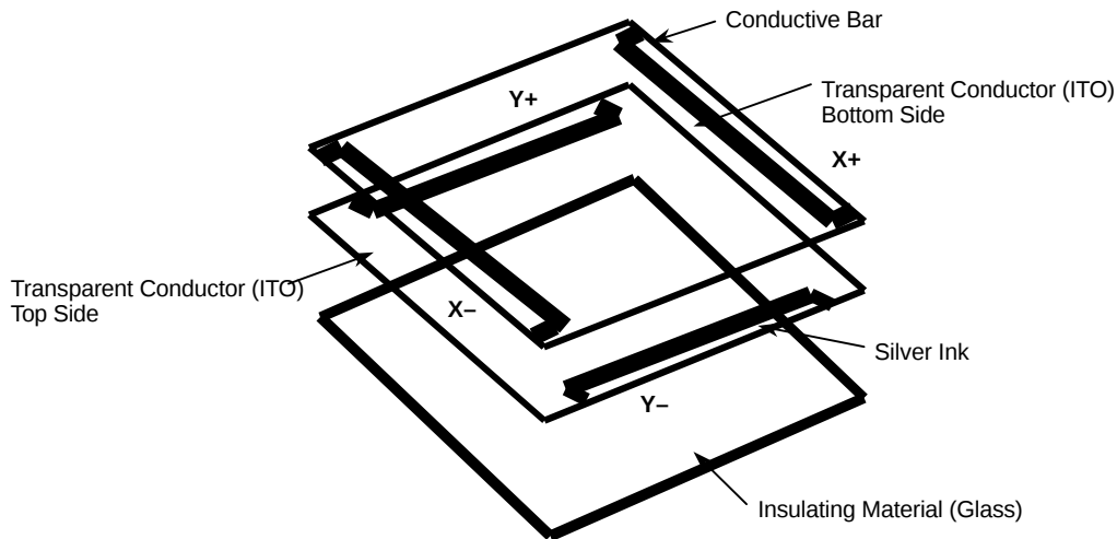
Figure 45. 4-wire Touch Screen Construction
