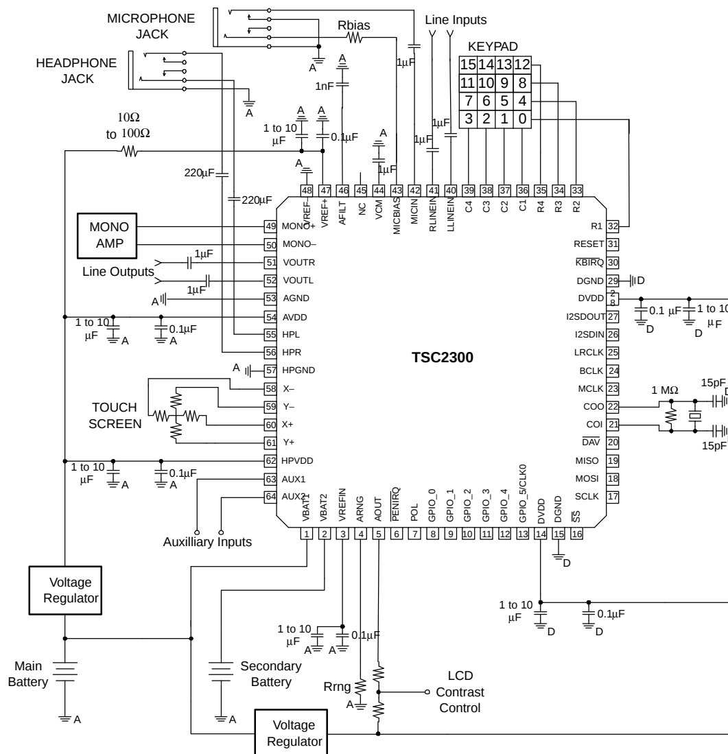
Figure 44. Typical Circuit Configuration.
