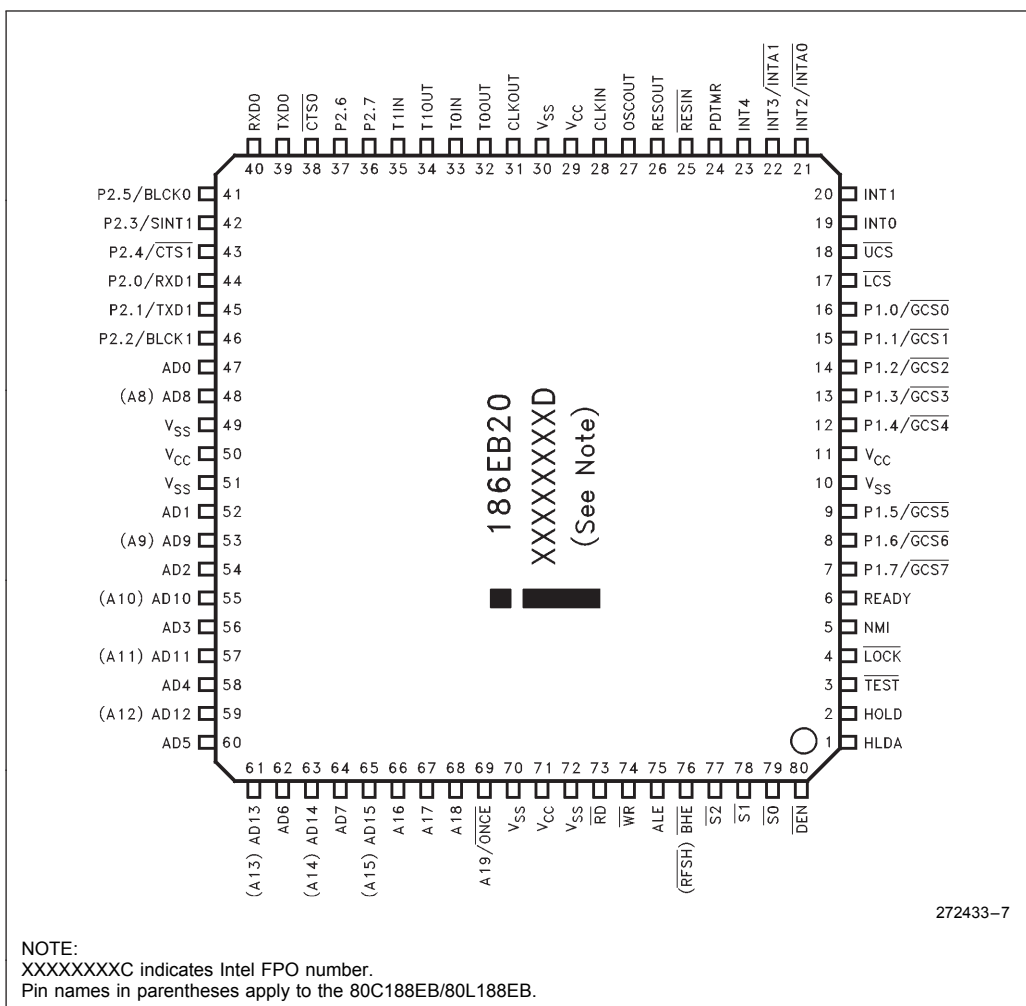
Figure 6. SQFP Package
