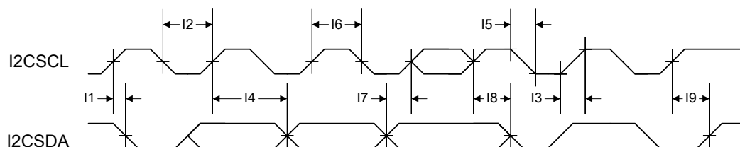
Figure 17-14. I 2 C Timing
