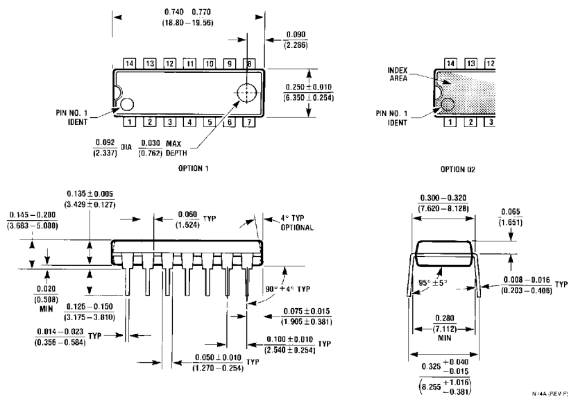
Molded Dual-In-Line Package (N) Order Number DM74ALS1035N Package Number N14A
