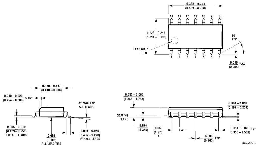
S.O. Package (M) Order Number DM74ALS1035M Package Number M14A
