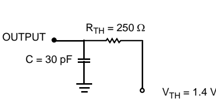
(b) Thévenin Equivalent (Load 1)
