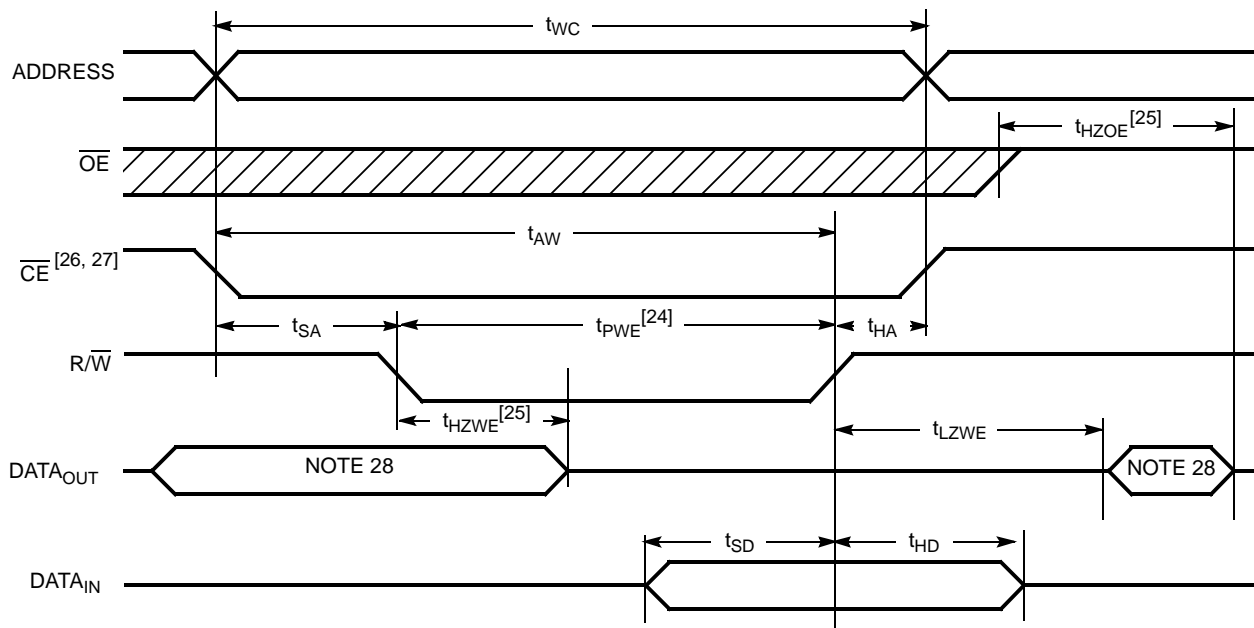
Figure 7. Write Cycle No. 2: \overline{CE} Controlled Timing [21, 22, 23, 29]
