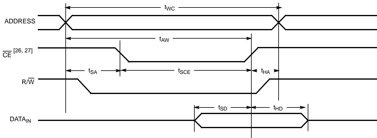
Figure 7. Write Cycle No. 2: \overline{CE} Controlled Timing [21, 22, 23, 29]
