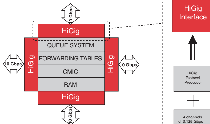
Nonblocking 8-Port Gigabit Ethernet Switch
