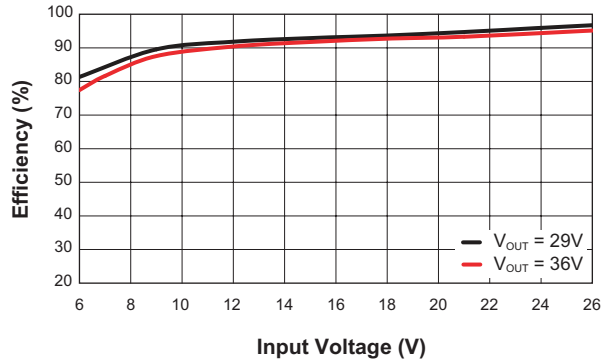
Boost Efficiency vs. Input Voltage ( L = 10\mu\text{H} ; V_{\text{CC}} = 4.7\text{V} ; \text{PWM} = V_{\text{CC}} ; F_{\text{SET}} = \text{GND} ; I_{\text{OUT}} = 360\text{mA} )
