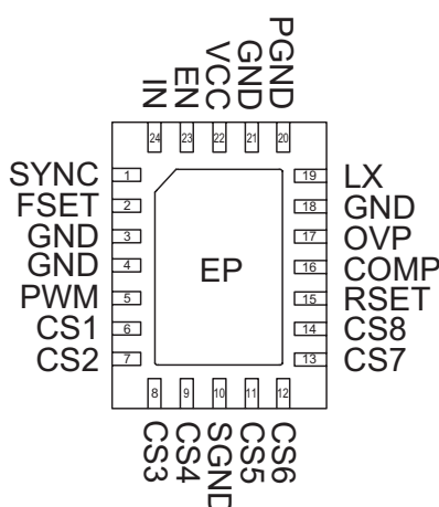
TQFN34-24 (Top View)
