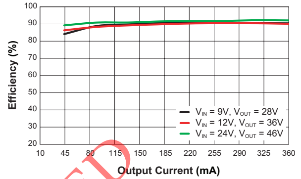
Boost Efficiency vs. Load Current ( L = 10\mu\text{H} ; V_{\text{CC}} = 4.7\text{V} ; \text{PWM} = V_{\text{CC}} ; F_{\text{SET}} = \text{GND} )
