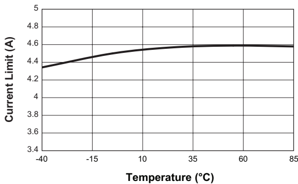
Low Side Switch Current Limit vs. Temperature ( V_{\text{IN}} = 5\text{V to } 26\text{V} )
