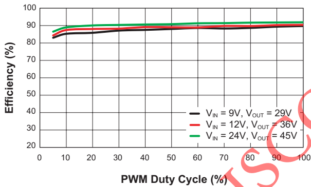
Boost Efficiency vs. PWM Duty Cycle ( L = 10\mu\text{H} ; V_{\text{CC}} = 4.7\text{V} ; F_{\text{SET}} = \text{GND} )
