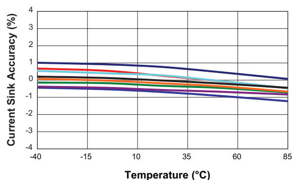
Current Sink Accuracy vs. Temperature ( V_{IN} = 12V ; V_{CSX} = 0.8V ; I_{CSX} = 21mA/\text{Channel} )
