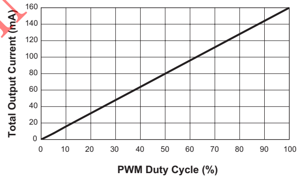
Output Current vs. PWM Duty Cycle ( V_{\text{IN}} = 12\text{V} ; I_{\text{CSx}} = 20\text{mA/ch} )
