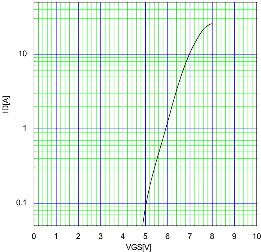
Typical Transfer Characteristic I_D=f(V_{GS}):80\text{ }\mu\text{s pulse test},V_{DS}=25V,T_{ch}=25\text{ }^{\circ}\text{C}
