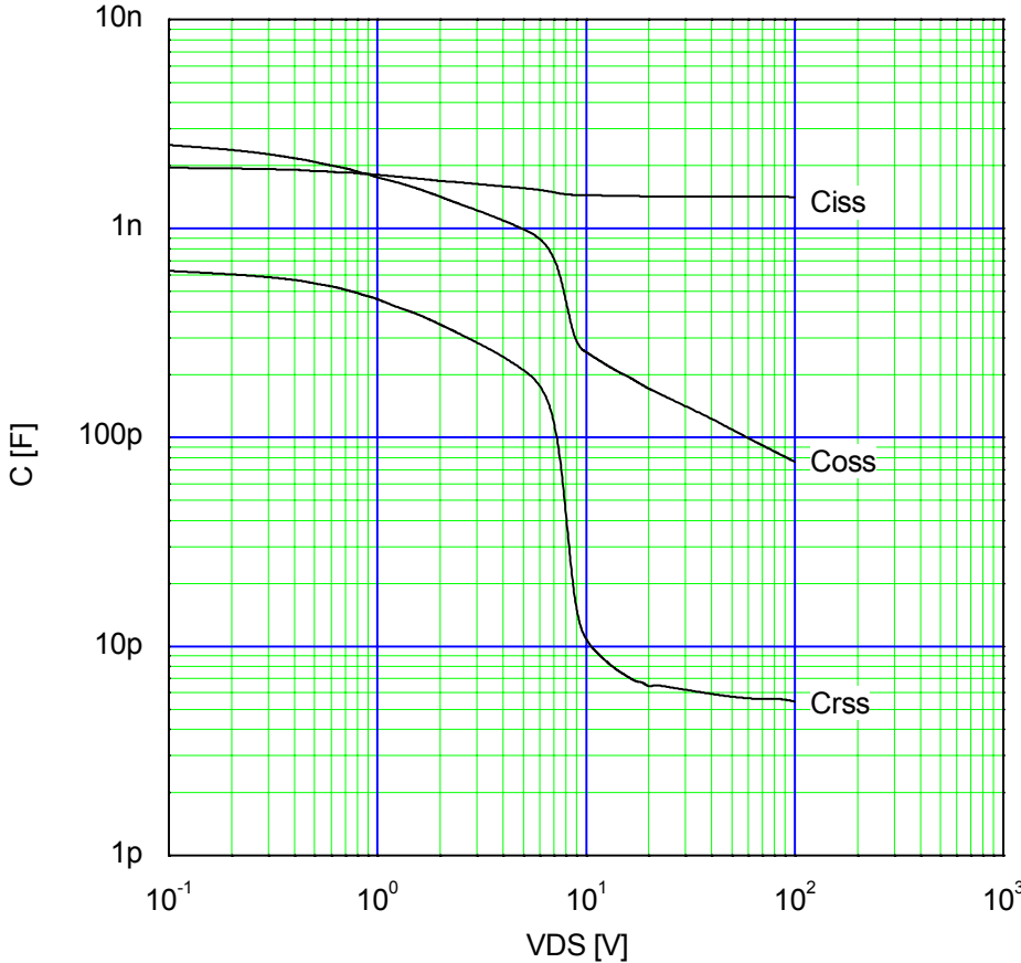
Typical Capacitance C=f(V_{DS}): V_{GS}=0V, f=1\text{MHz}
