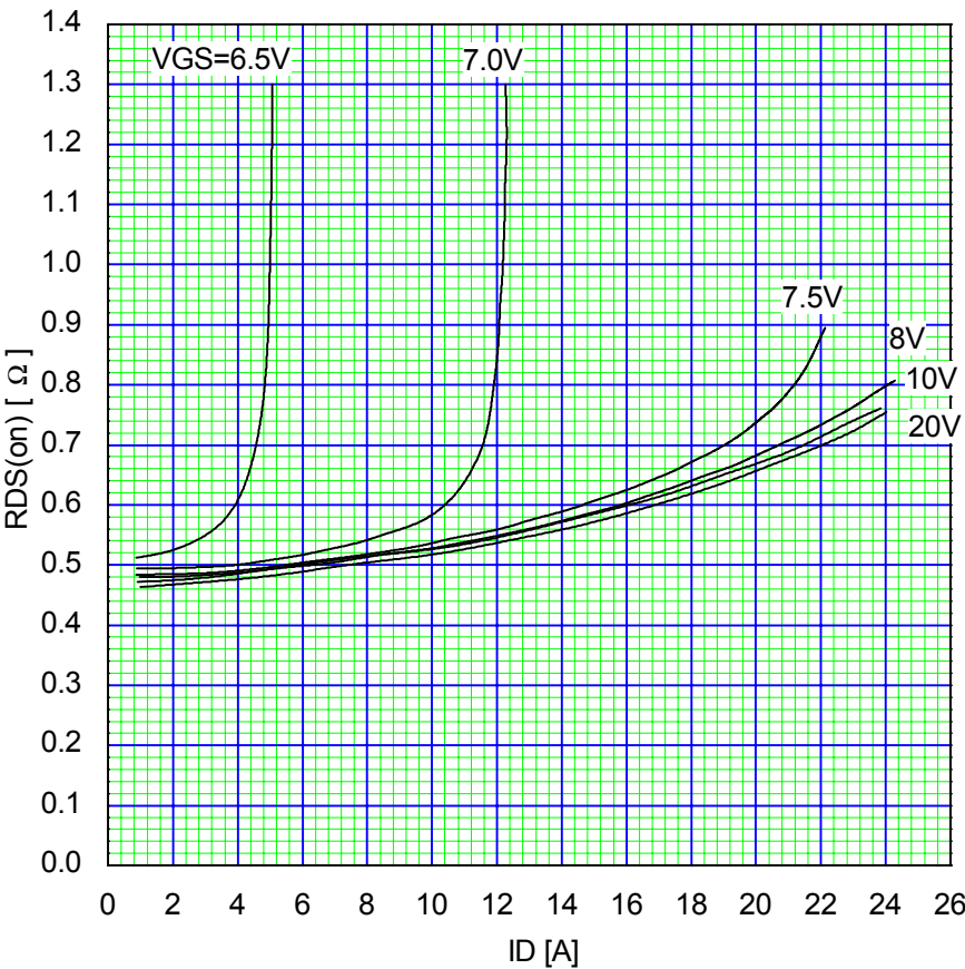
Typical Drain-Source on-state Resistance R_{DS(on)}=f(I_D) :80 \mu s pulse test, T_{ch}=25\text{ }^{\circ}C
