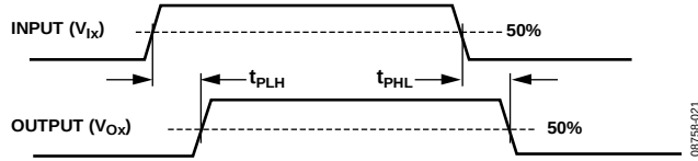
Figure 22. Propagation Delay Parameters
