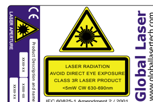
Class 3R Laser Label
