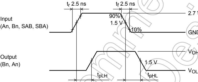
Figure 2 t_{pLH} , t_{pHL}
