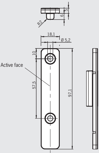
Dimension drawing
