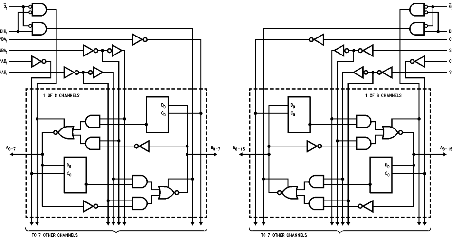
Logic Diagram
