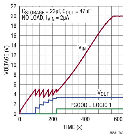
LTC3588-1 3.3V Regulator Start-Up Profile
