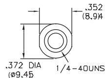
Dress Nut
