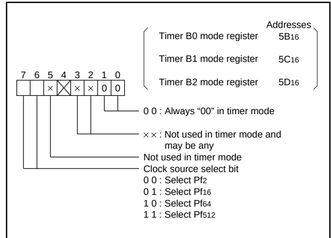
Fig. 36 Timer Bi mode register bit configuration during timer mode
