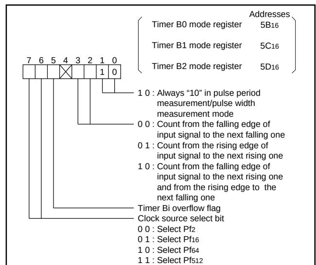
Fig. 38 Timer Bi mode register bit configuration during pulse period measurement/pulse width measurement mode
