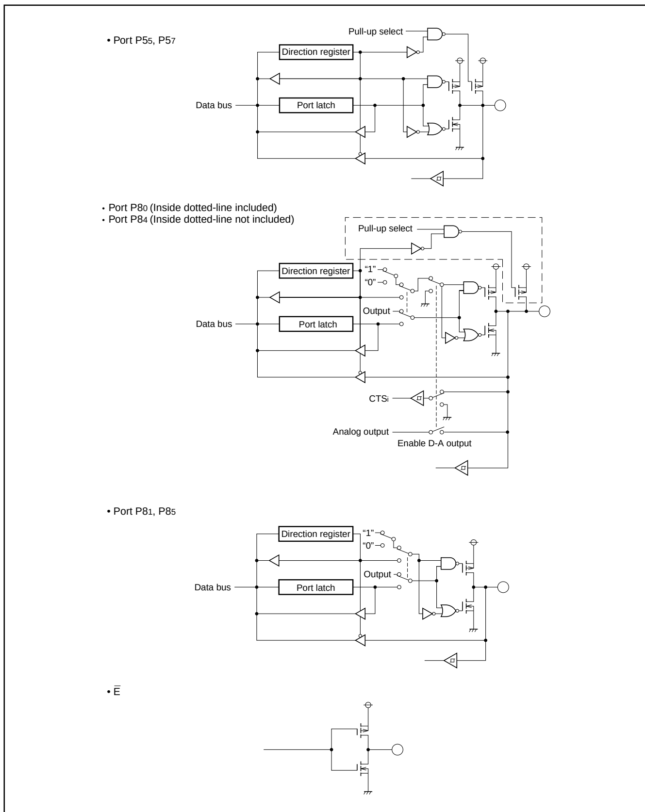
Fig. 79 Block diagram for ports P0 to P8 in single-chip mode and \bar{E} output (2)
