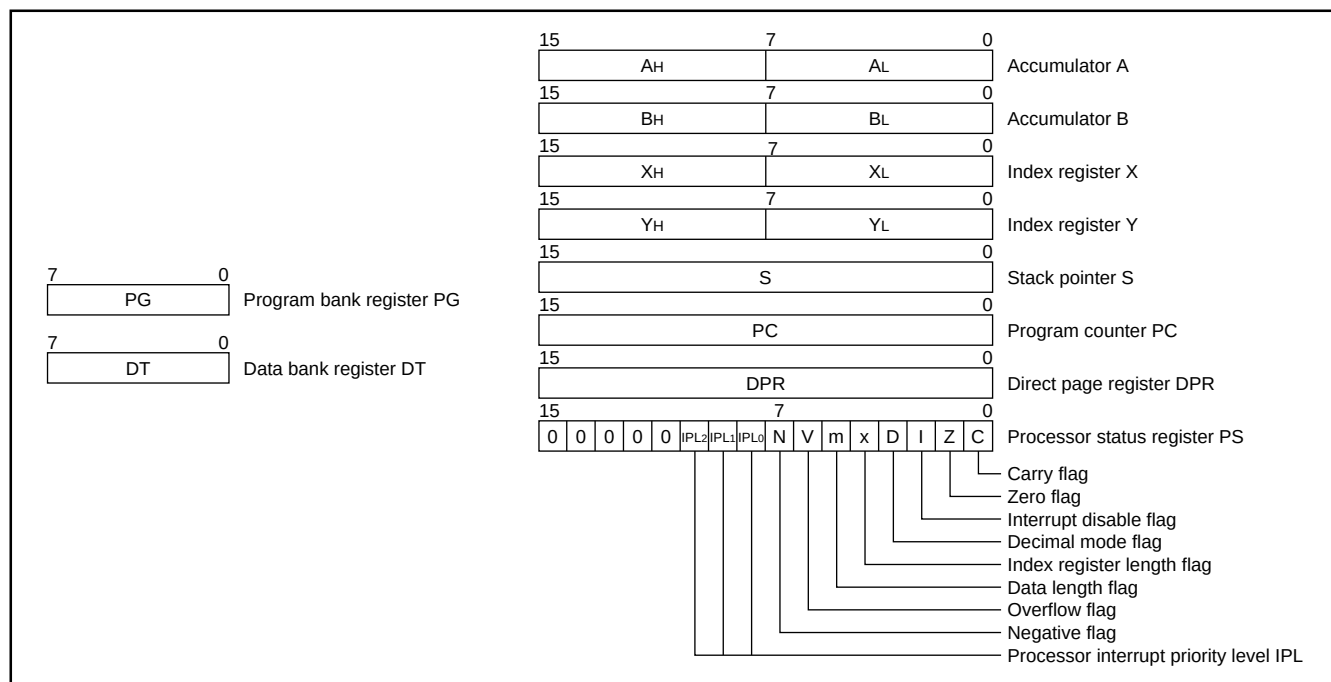
Fig. 3 Register structure
