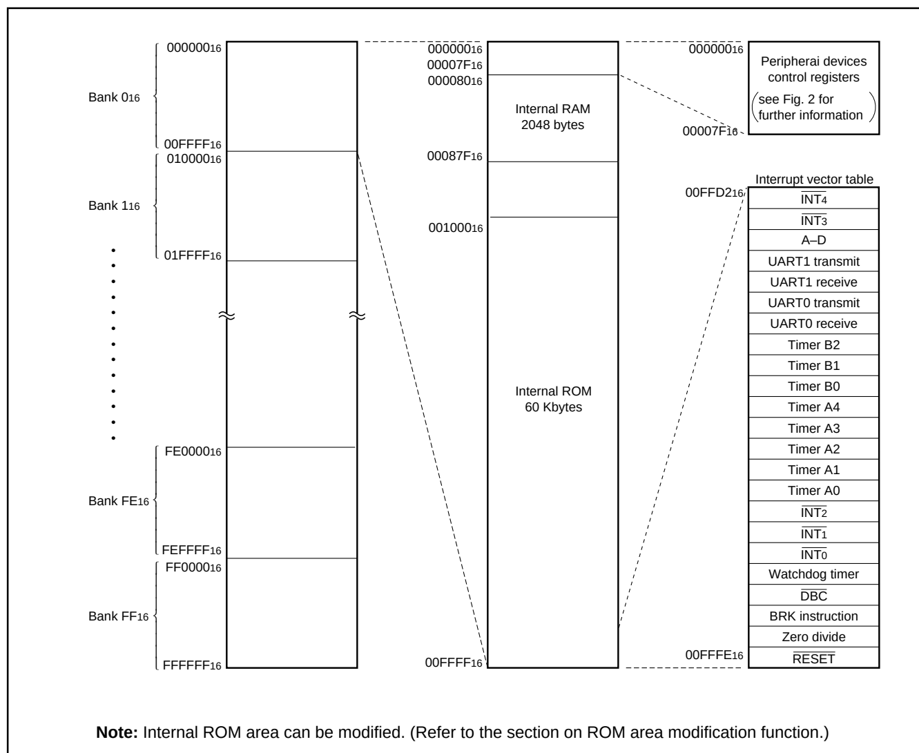
Fig. 1 Memory map
