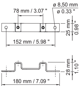
Backstrap bracket
