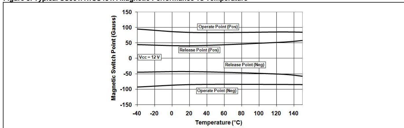
Figure 3. Typical SS351AT/SS451A Magnetic Performance vs Temperature
