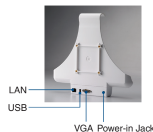
I/O Ports for MICA-101-VCRE
