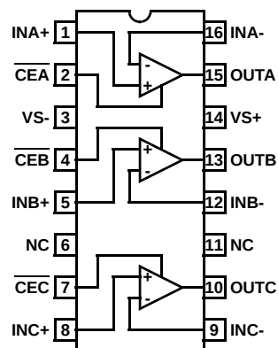
EL5300 (16 LD QSOP) TOP VIEW
