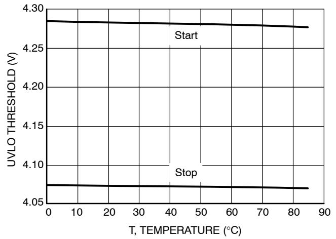
Figure 5. UVLO Threshold vs. Temperature
