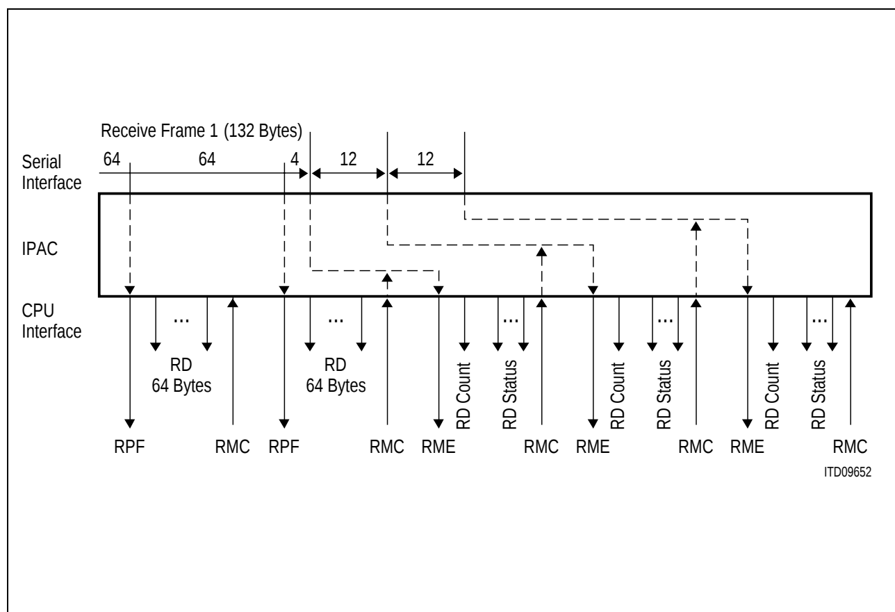
Figure 85 Interrupt Driven Reception Sequence Example
