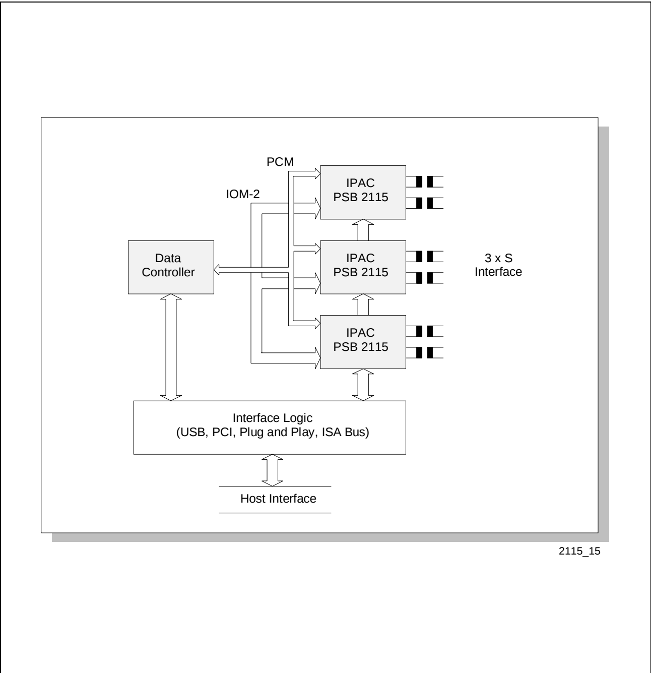
Figure 8 Multiline PC-Adapter
