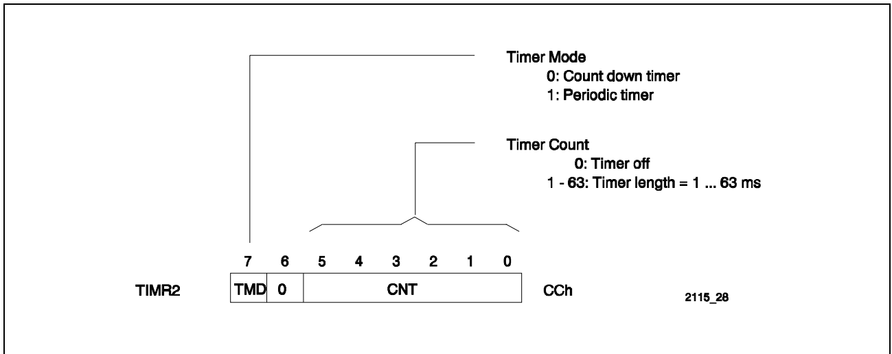
Figure 49 Timer 2 Register
