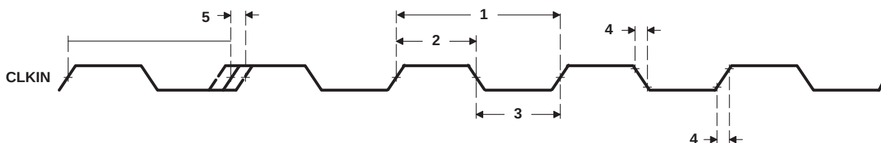
Figure 4–5. CLKIN Timing
