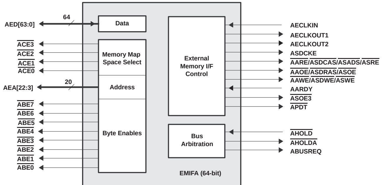
Figure 1–7. Peripheral Signals
