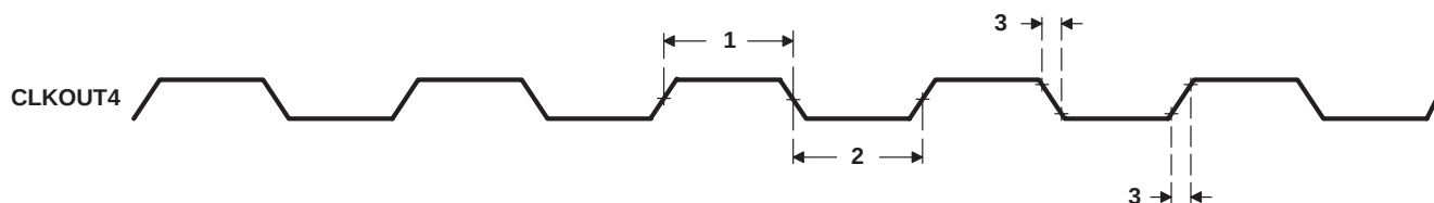
Figure 4-6. CLKOUT4 Timing
