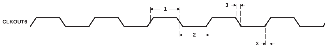
Figure 4-7. CLKOUT6 Timing
