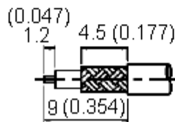
Stripping Dimension
