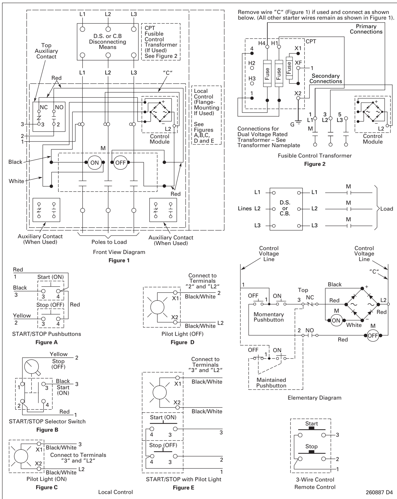
Figure 5-4. Magnetically Latched Combination Contactors
