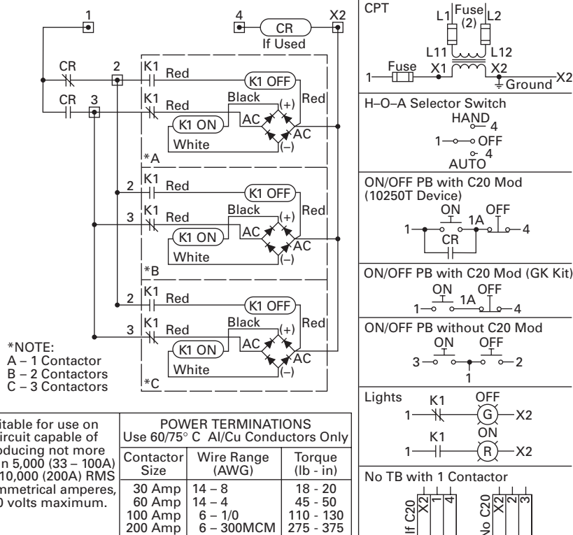
Figure 5-2. Typical Wiring Diagram — Magnetically Latched
