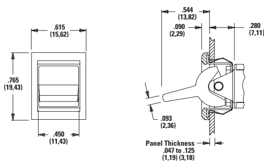
J61 Lever with Frame, Snap-in
