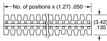
THROUGH-HOLE
