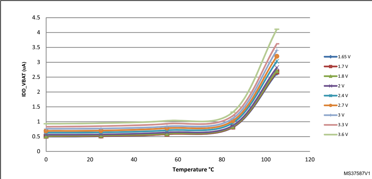
Figure 21. Typical V_{BAT} current consumption (RTC ON/BKP SRAM OFF and LSE in medium high drive mode)
