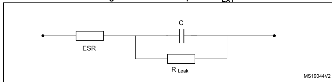
Figure 18. External capacitor C_{\text{EXT}}
