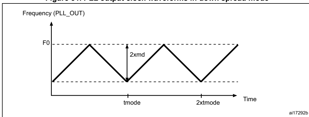
Figure 31. PLL output clock waveforms in down spread mode
