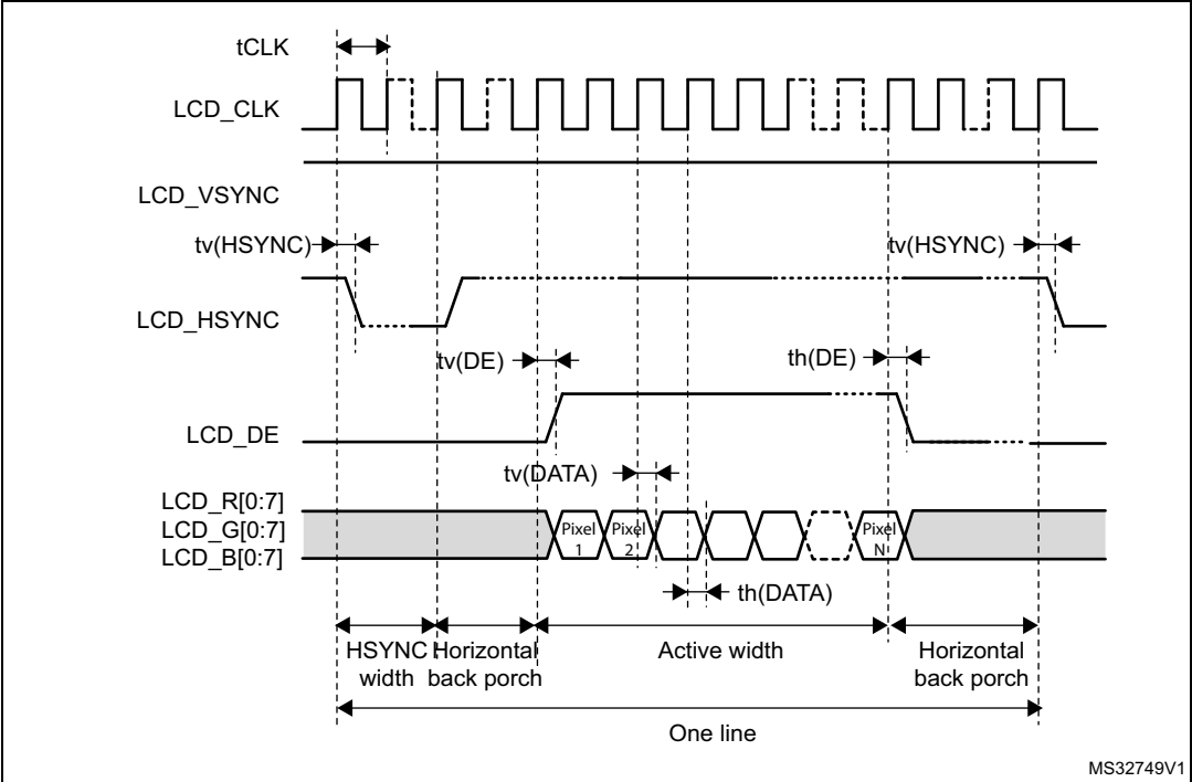
Figure 69. LCD-TFT horizontal timing diagram
