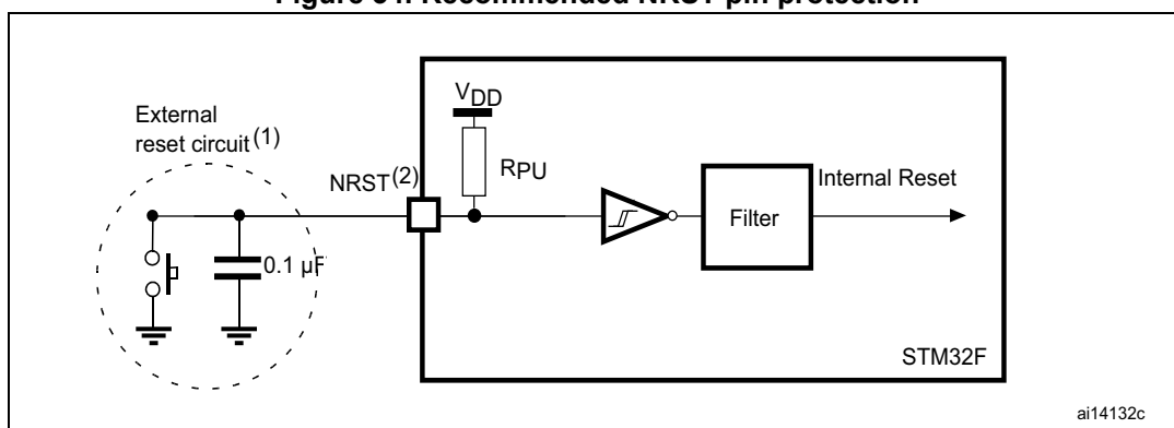
Figure 34. Recommended NRST pin protection
